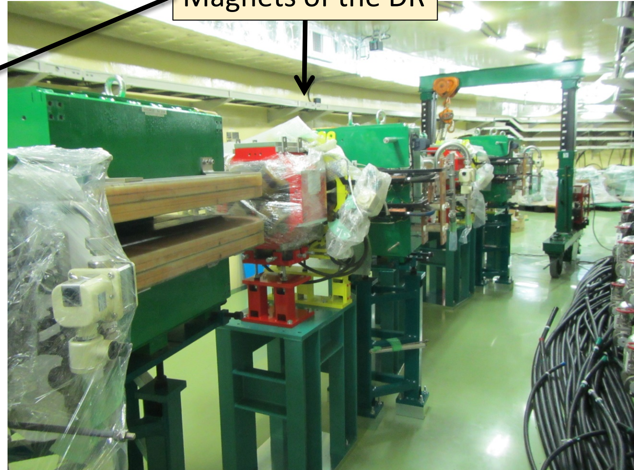
Magnets of the DR
