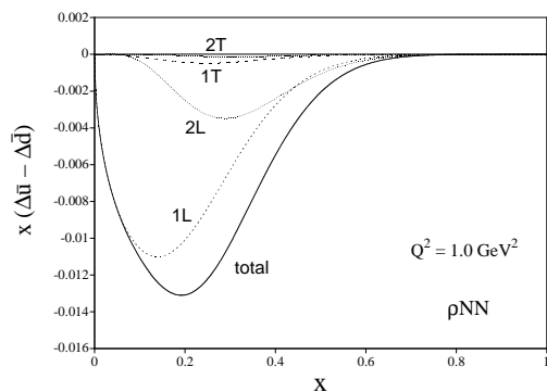
FIG. 7: \Delta\bar{u} - \Delta\bar{d} distributions from the \rho NN process at Q^2=1 \text{GeV}^2 . The 1L , 2L , 1T , and 2T type contributions and their summation are shown.
