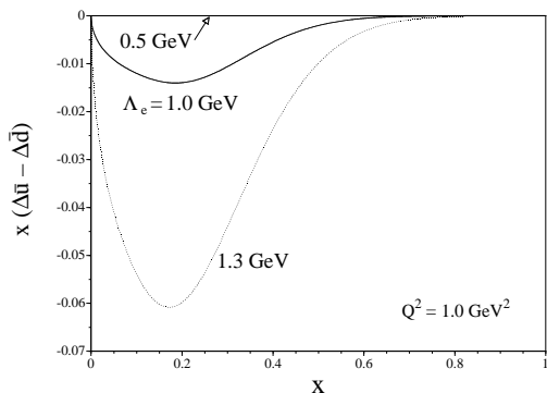
FIG. 11: Cutoff dependence of \Delta\bar{u} - \Delta\bar{d} is shown at Q^2=1 \text{GeV}^2 by taking \Lambda_e=0.5, 1.0, \text{ and } 1.3 \text{GeV} .
