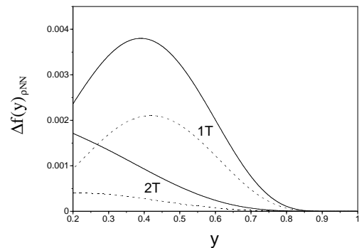
FIG. 3: Meson momentum distributions \Delta f_{1T}(y) and \Delta f_{2T}(y) from the \rho NN process. The solid and dashed curves are obtained at Q^2=1 and 2 \text{ GeV}^2 , respectively, with x=0.2 .
