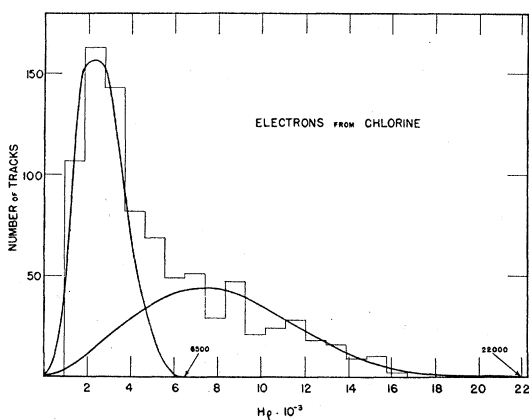
FIG. 7. Distribution histogram for the electrons emitted from activated chlorine. The general shape of this curve is much more skewed than a simple K-U curve. As can be seen from Fig. 8 one may resolve this curve into the sum of two simple K-U curves. The upper limits so found are at 6500H\rho and 22,000H\rho .
