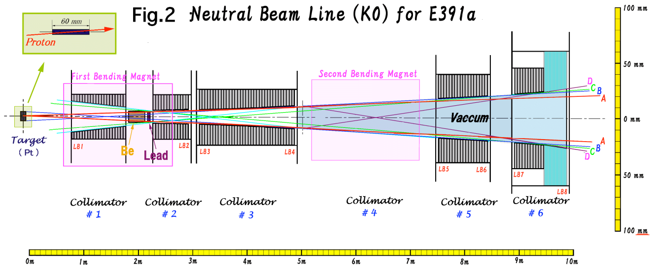
FIG. 2 : PROFILES OF NEUTRON AND PHOTON AT KU BEAM LINE
