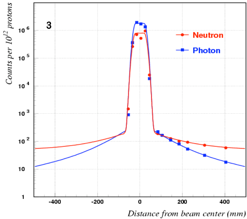
FIG. 2 : PROFILES OF NEUTRON AND PHOTON AT KU BEAM LINE
