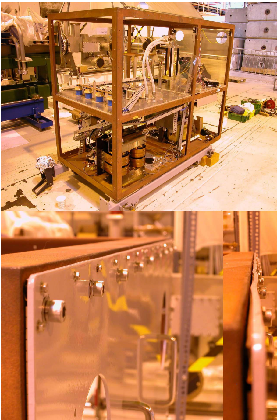
Photo 1: New RF shield panels putted on RF chassis.
