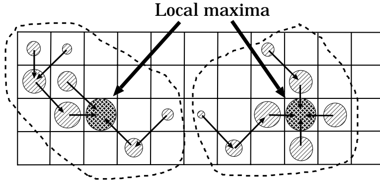
Figure A.1: A schematic view of the island clustering based on energy gradients. The squares indicate a unit of clustering: towers for tower-islands or cells for cell-islands. The size of circles shows a size of the energy deposit in the unit. In this figure, two islands are formed, each of which is surrounded with a dashed line.
