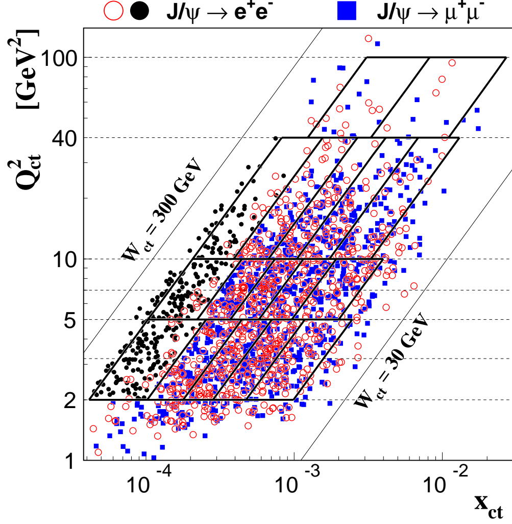
Figure 8.1: Bin definition (bold-solid lines) and the final data events of the J/\psi \rightarrow e^+e^- (circles) and J/\psi \rightarrow \mu^+\mu^- (squares) candidates. The closed circles indicate the one-track sample.
