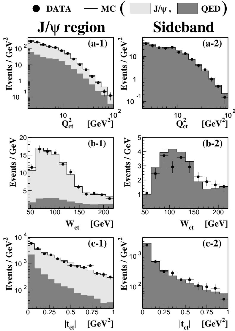
Figure 7.12: Comparisons between the data and MC on kinematical variables (a,b,c-1) in the J/\psi mass window and (a,b,c-2) in the sideband ( 4 < M_{l+l-} < 8 GeV).
