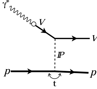
Figure 3.2: A diagram for exclusive production of the vector meson V , based on the VDM and the Regge theory. IP indicates a Pomeron trajectory.
