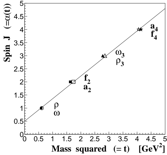
Figure 3.4: An example of the Chew-Frautschi plot and the Regge trajectory (solid line).
