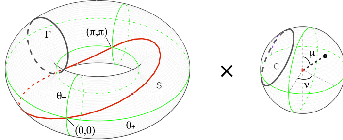
Fig. 1. U(2) parameter space as a product of the torus T^2 determining the spectrum (the spectral space is its half T^2/Z_2 which is a Möbius strip) and the isospectral sphere S^2 .
