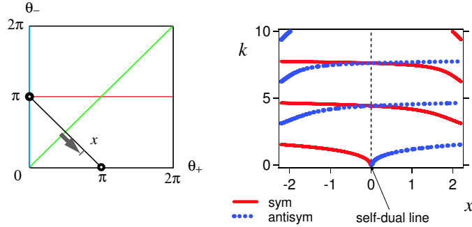
Fig. 2. Spectra of two systems with a singularity placed at the centre of an infinite well, where k is the momentum with the energy E = \hbar k^2/(2m) . The spectra, drawn as a function of x on the torus, are identical for x and -x , that is, for (\theta_+, \theta_-) and (\theta_-, \theta_+) .
