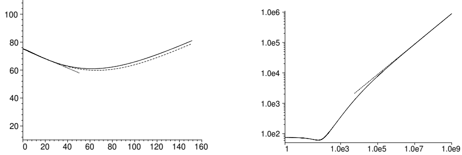
Fig. 7. Left: The dimensionless net force \frac{1}{2\mathcal{E}} \Delta F(t) for N = 100 , in the temperature region 0 < t < 160 , obtained by a numerical computation (solid line), and approximated by (47) (dotted line), and by (48) using (49) (dashed line). Right: The dimensionless net force \frac{1}{2\mathcal{E}} \Delta F(t) for N = 100 , obtained by a numerical computation (solid line), and approximated for high temperatures with (56) (dashed line). The figure is double logarithmic.
