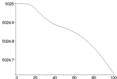
Fig. 8. The dimensionless net force \frac{l}{2\epsilon}\Delta F(t) in the fermionic case, for N = 100 , in the low-temperature region.
