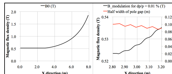
Fig. 2. An example of magnetic field configuration to energize 0.1 GeV proton up to 1.1 GeV. Left: magnetic field configuration to satisfy the isochronous condition. Right: magnetic field configuration to satisfy the isochronous condition with phase stability for dp/p = 0.01\% .
