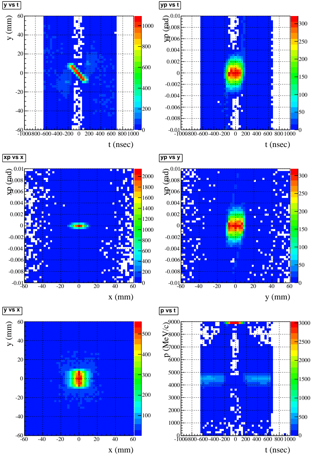
FIG. 9: Outlet of the collimator. Upper left: time vs y . Upper right: time vs y' . Middle left: Phase distribution ( x - x' ). Middle right: Phase distribution ( y - y' ). Lower left: Beam profile ( x - y ). Lower right: time vs momentum.
