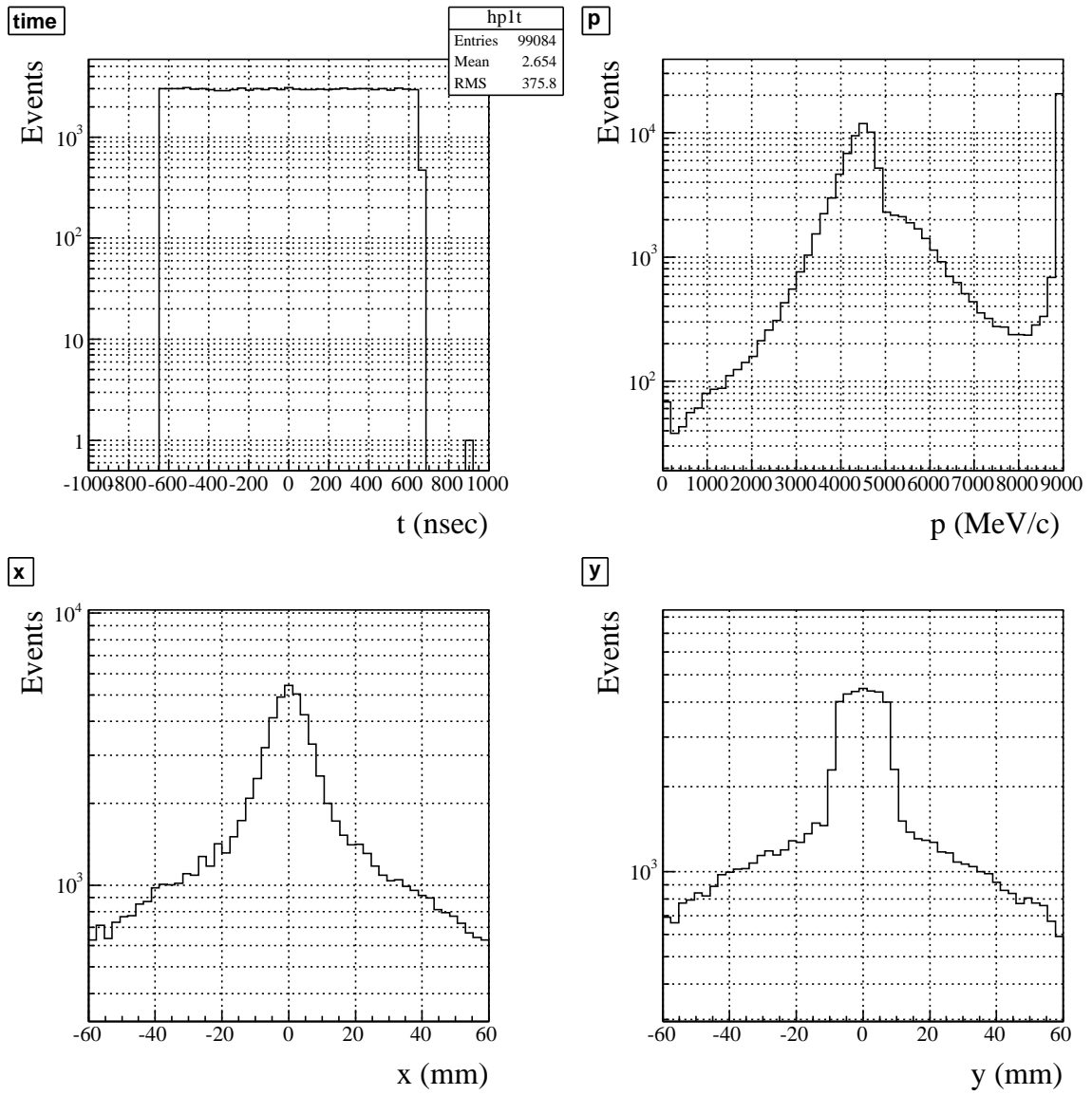
FIG. 8: Collimator outlet. Upper left: time sepctrum. Upper right: Momentum spectrum. Lower left: Beam profile in x axis. Lower right: Beam profile in y axis.
