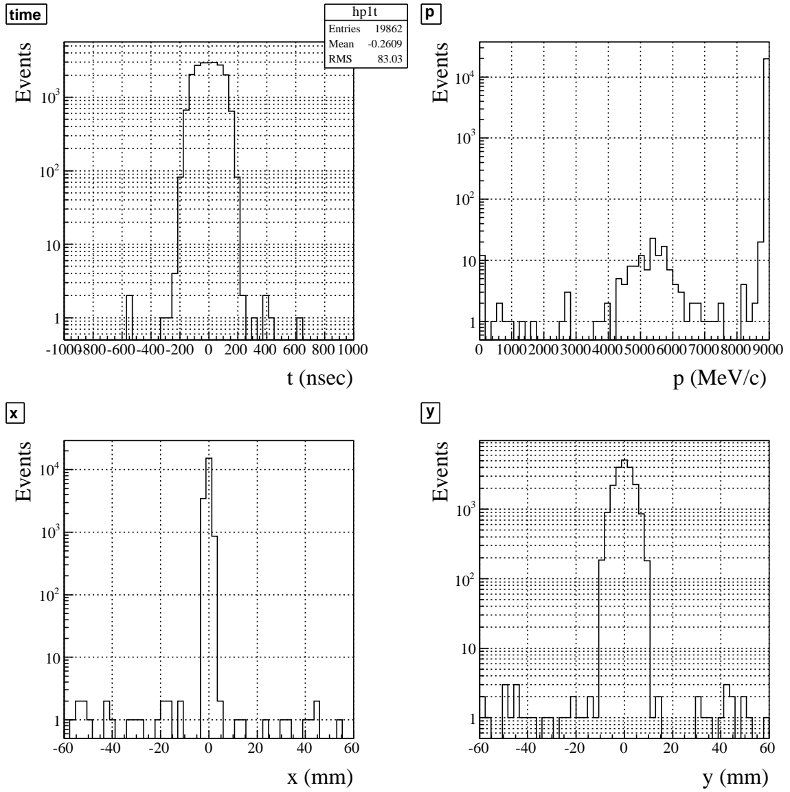
FIG. 12: Outlet of the final focus section. Upper left: time spectrum. Upper right: Momentum spectrum. Lower left: Beam profile in x axis. Lower right: Beam profile in y axis.
