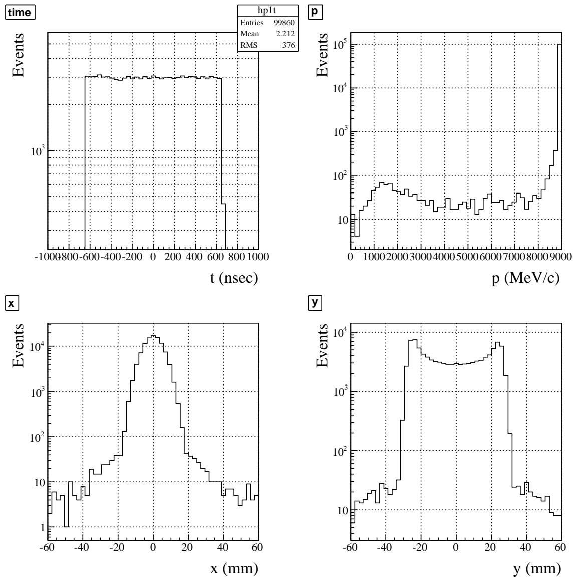
FIG. 6: Inlet of the collimator. Upper left: time sepctrum. Upper right: Momentum spectrum. Lower left: Beam profile in x axis. Lower right: Beam profile in y axis.
