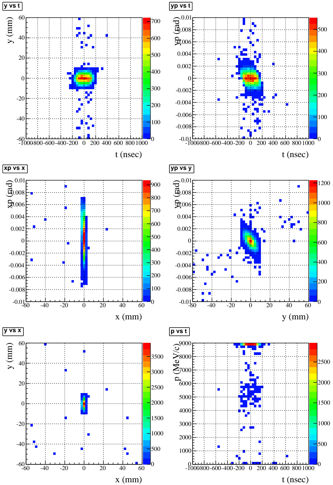
FIG. 13: Outlet of the final-focus section. Upper left: time vs y . Upper right: time vs y' . Middle left: Phase distribution ( x - x' ). Middle right: Phase distribution ( y - y' ). Lower left: Beam profile ( x - y ). Lower right: time vs momentum.
