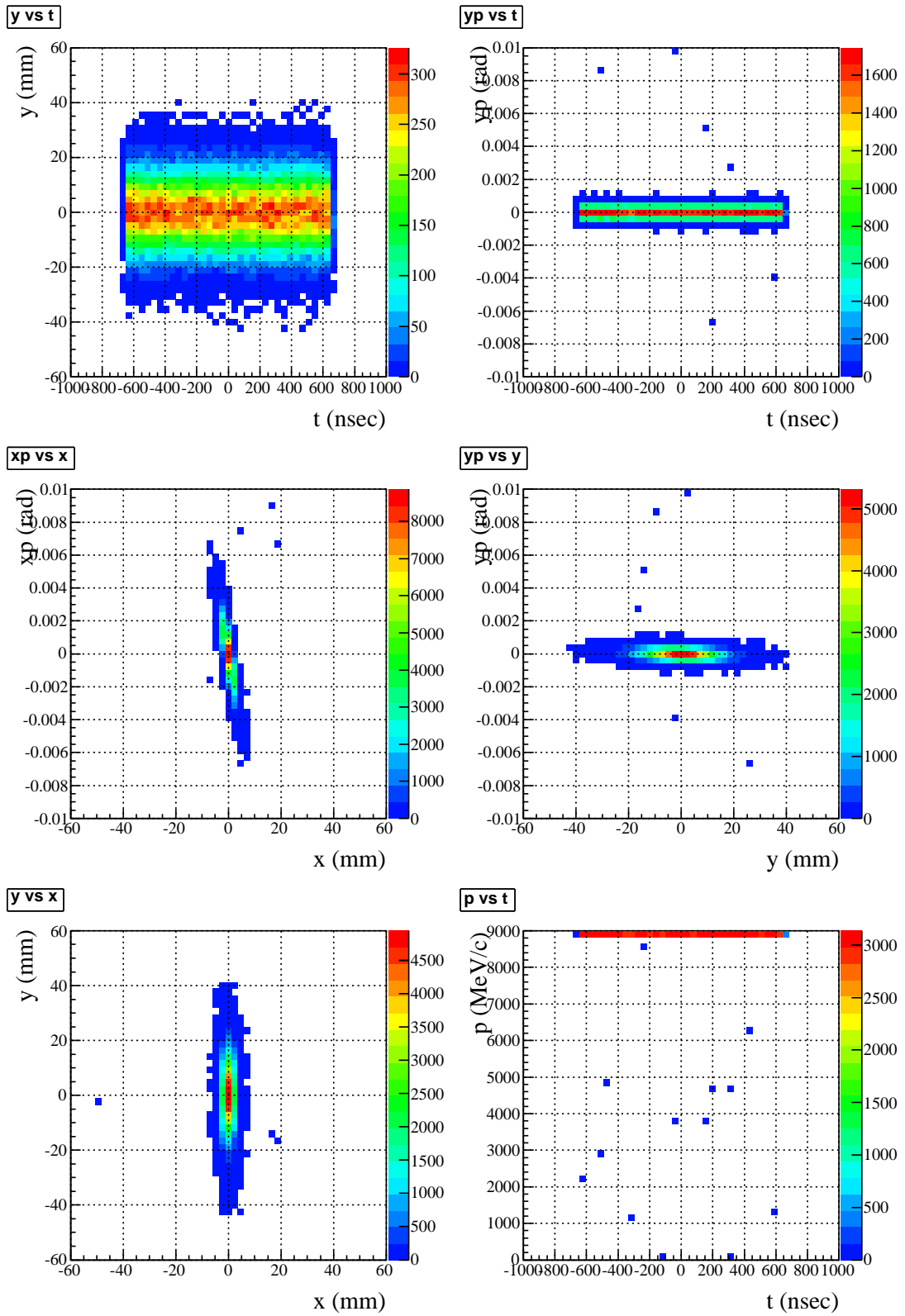
FIG. 5: Inlet of the 1st AC-dipole. Upper left: time vs y . Upper right: time vs y' . Middle left: Phase distribution ( x - x' ). Middle right: Phase distribution ( y - y' ). Lower left: Beam profile ( x - y ). Lower right: time vs momentum.
