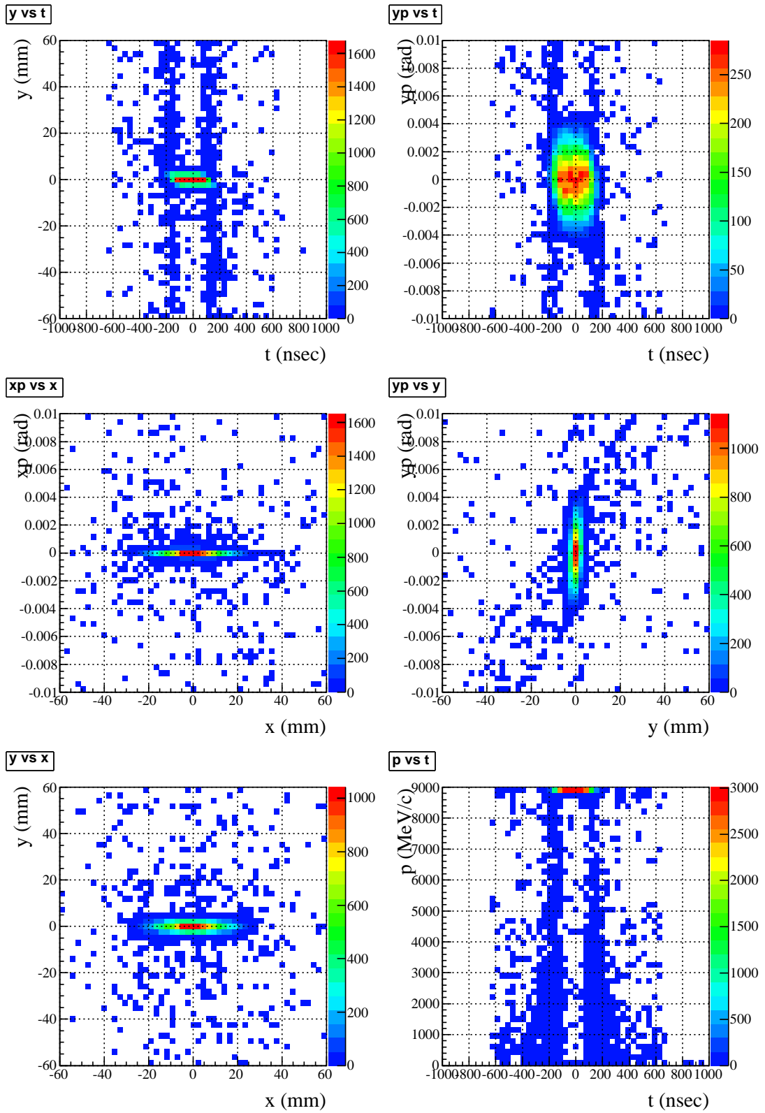
FIG. 11: Outlet of the AC-dipole section (inlet of the final-focus section). Upper left: time vs y . Upper right: time vs y' . Middle left: Phase distribution ( x - x' ). Middle right: Phase distribution ( y - y' ). Lower left: Beam profile ( x - y ). Lower right: time vs momentum.
