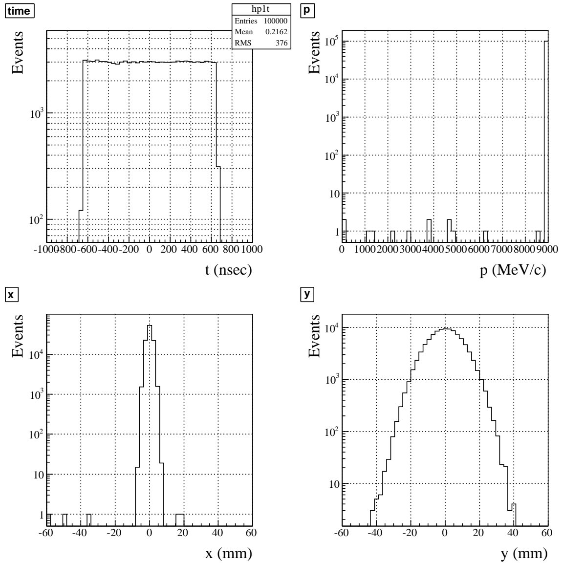
FIG. 4: Inlet of the 1st AC-dipole. Upper left: time spectrum. Upper right: Momentum spectrum. Lower left: Beam profile in x axis. Lower right: Beam profile in y axis.
