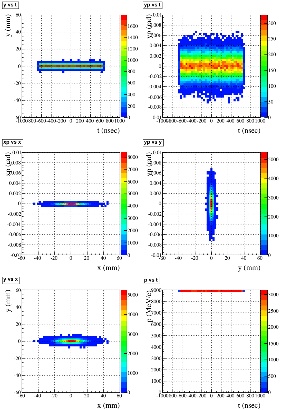
FIG. 3: Inlet of the AC-dipole section. Upper left: time vs y . Upper right: time vs y' . Middle left: Phase distribution ( x - x' ). Middle right: Phase distribution ( y - y' ). Lower left: Beam profile ( x - y ). Lower right: time vs momentum.
