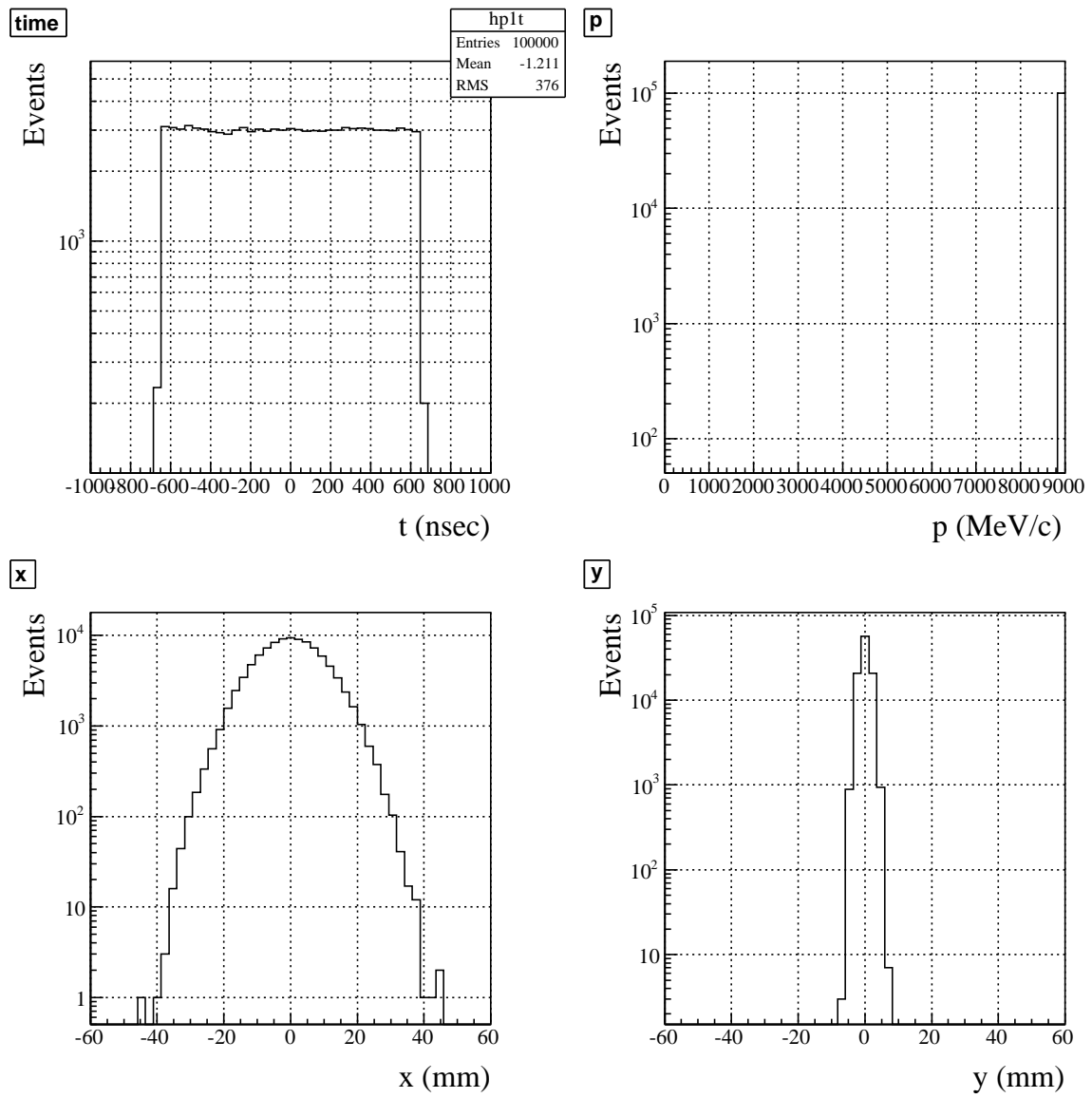
FIG. 2: Inlet of the AC-dipole section. Upper left: time spectrum. Upper right: Momentum spectrum. Lower left: Beam profile in x axis. Lower right: Beam profile in y axis.
