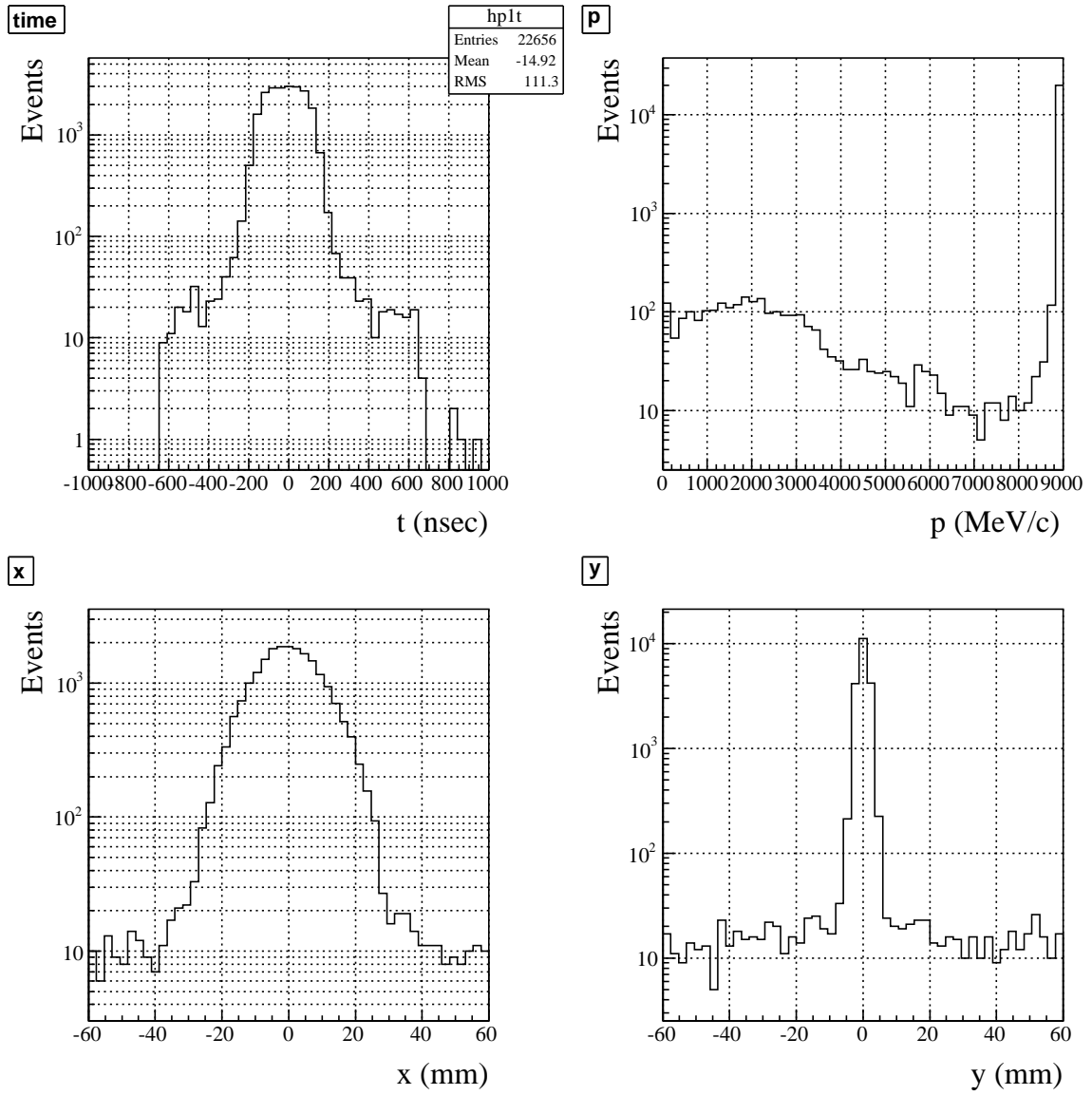
FIG. 10: Outlet of the AC-dipole section (inlet of the final-focus section). Upper left: time sepctrum. Upper right: Momentum spectrum. Lower left: Beam profile in x axis. Lower right: Beam profile in y axis.
