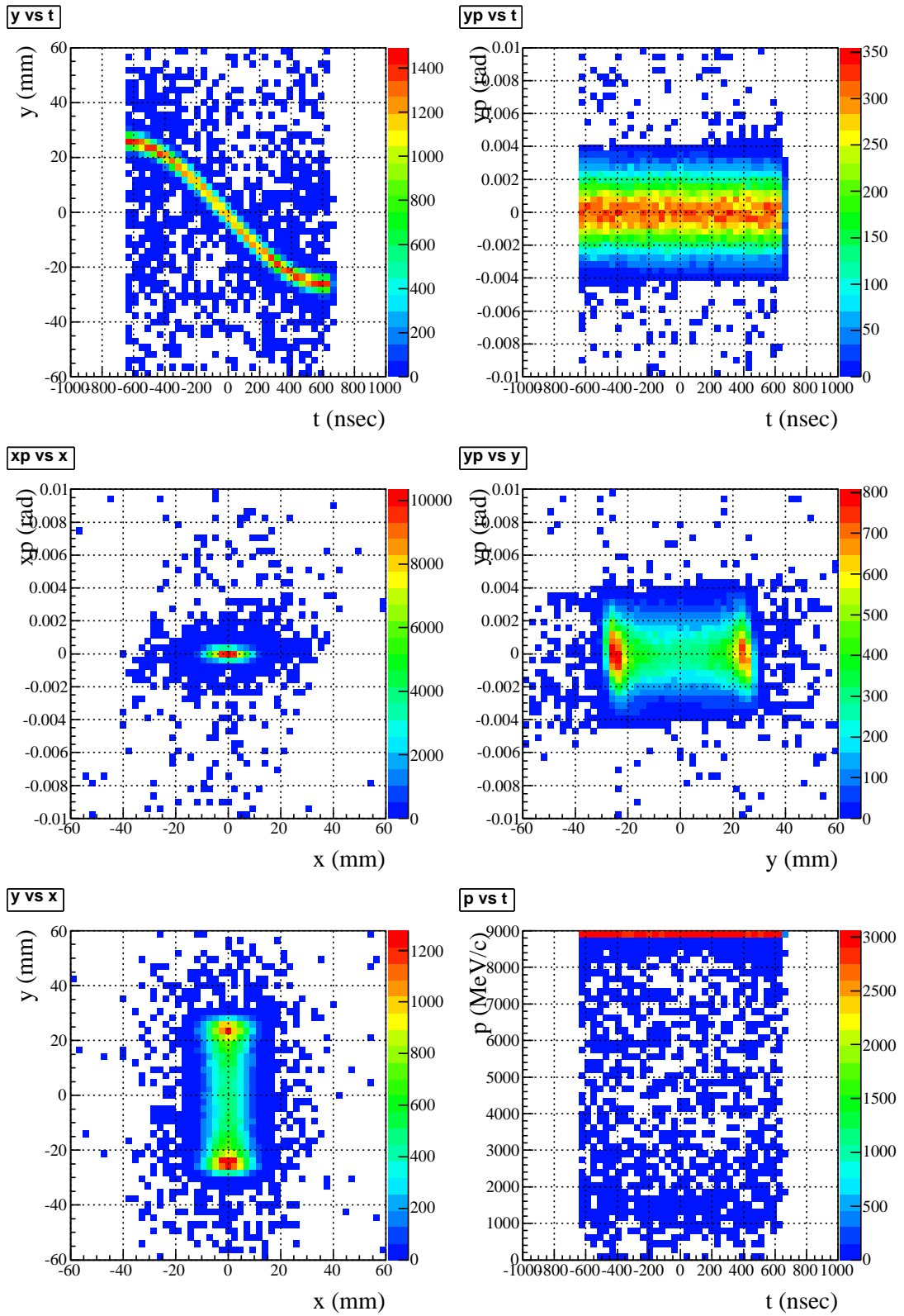
FIG. 7: Inlet of the collimator. Upper left: time vs y . Upper right: time vs y' . Middle left: Phase distribution ( x - x' ). Middle right: Phase distribution ( y - y' ). Lower left: Beam profile ( x - y ). Lower right: time vs momentum.
