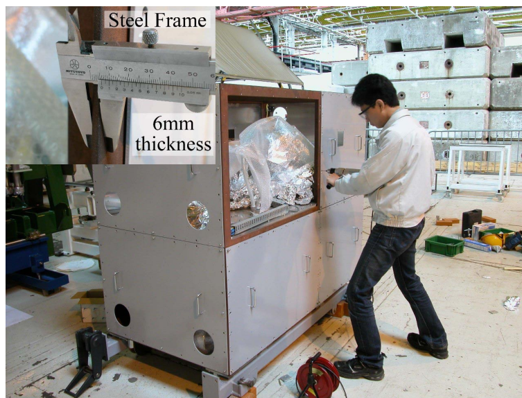
Photo 2: Work for new RF shield panels
