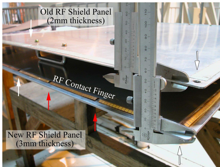
Photo 1: New RF shield panel comparing with old one
