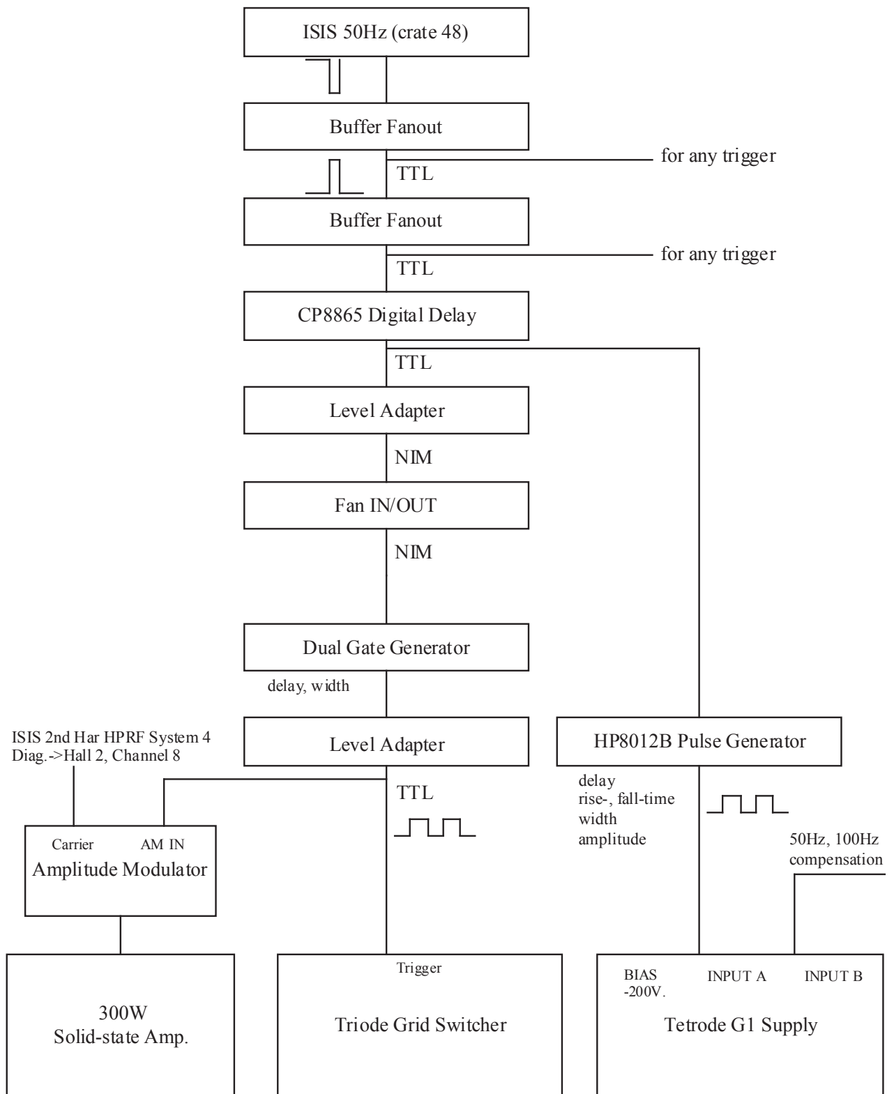
Figure 3: LOI timing system for grid switching and triggers
