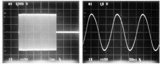
a) 5\text{V}/\text{div} \times 1000 , 1\text{ms}/\text{div} . b) 5\text{V}/\text{div} \times 1000 , 50\text{ns}/\text{div} . Figure 11: Waveforms of gap voltage of 12\text{kV} at 5.91\text{MHz} .
